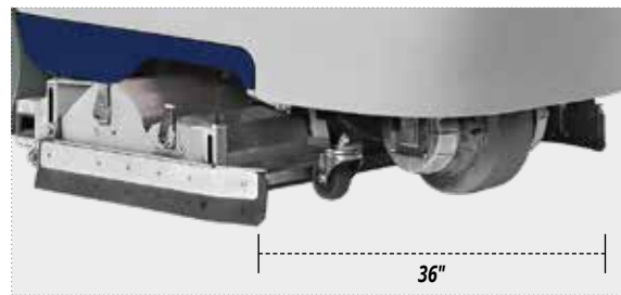
Cylindrical brush (BC)
